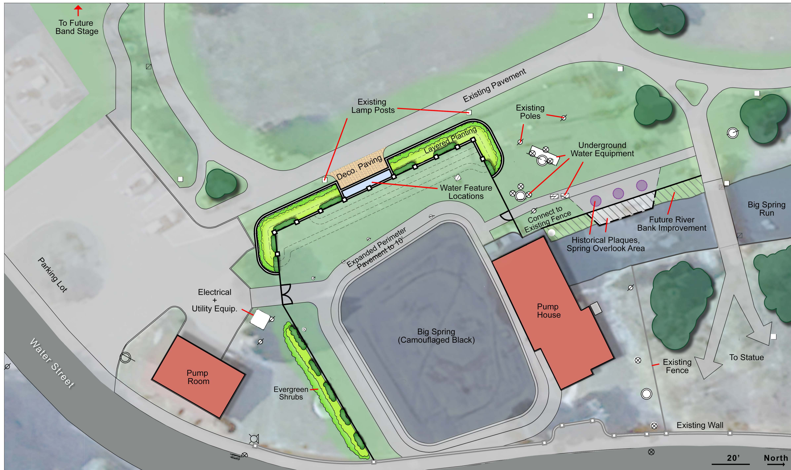
Talleyrand Park Big Spring Landscape Conceptual Study - Site Plan Diagram
